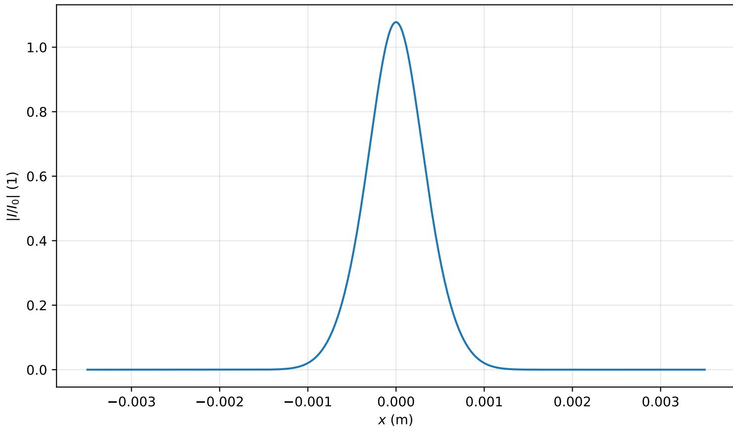
Intensity profile I(x, y = 0, z = 0.557m)/I_0 , P_{in}=0.6P_{cr} , artificial time
